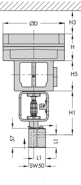
Type 3510-7 as angle valve with female thread
